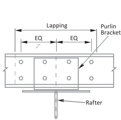
Z Purlin Overlapping
