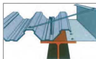
TYPICAL SIDE DETAIL
